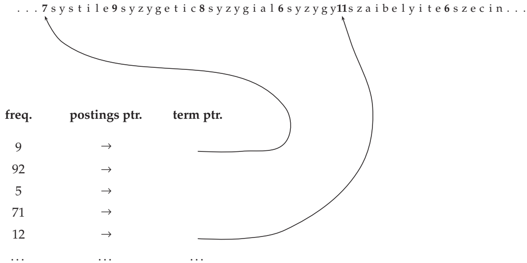
Figure 5.5 Blocked storage with four terms per block. The first block consists of systile, syzygetic, syzygial, and syzygy with lengths of seven, nine, eight, and six characters, respectively. Each term is preceded by a byte encoding its length that indicates how many bytes to skip to reach subsequent terms.
