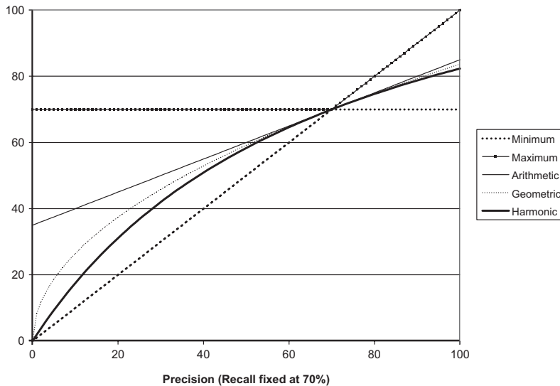
Figure 8.1 Graph comparing the harmonic mean to other means. The graph shows a slice through the calculation of various means of precision and recall for the fixed recall value of 70%. The harmonic mean is always less than either the arithmetic or geometric mean, and often quite close to the minimum of the two numbers. When the precision is also 70%, all the measures coincide.
