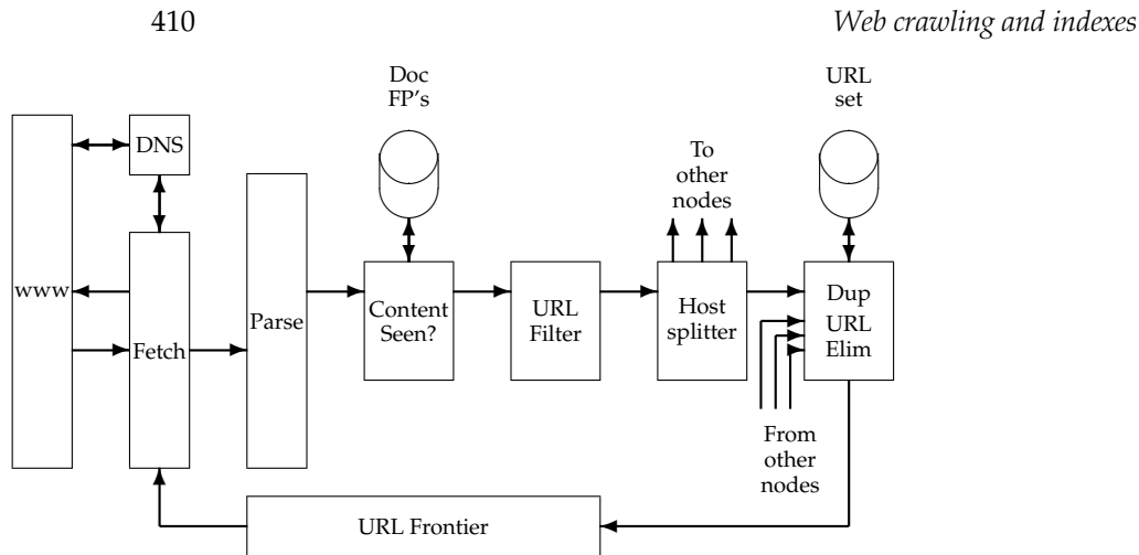
Figure 20.2 Distributing the basic crawl architecture.
