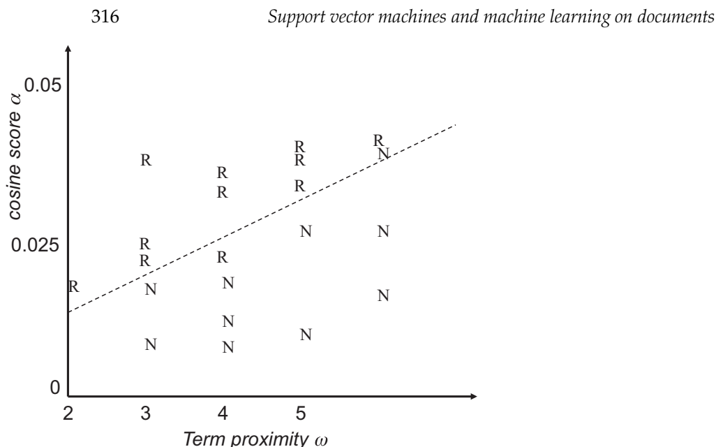
Figure 15.7 A collection of training examples. Each R denotes a training example labeled relevant and each N is a training example labeled nonrelevant .
