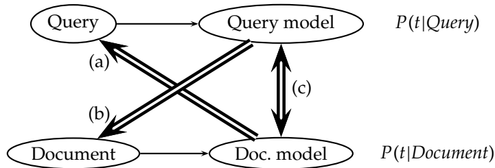
Figure 12.5 Three ways of developing the language modeling approach. (a) Query likelihood. (b) Document likelihood. (c) Model comparison.
