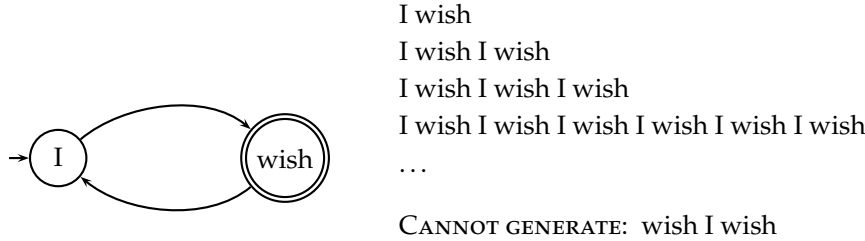
Figure 12.1 A simple finite automaton and some of the strings in the language it generates. → shows the start state of the automaton and a double circle indicates a (possible) finishing state.
