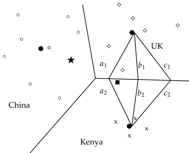
Figure 14.3 Rocchio classification.
