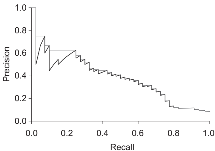
Figure 8.2 Precision–recall graph.
