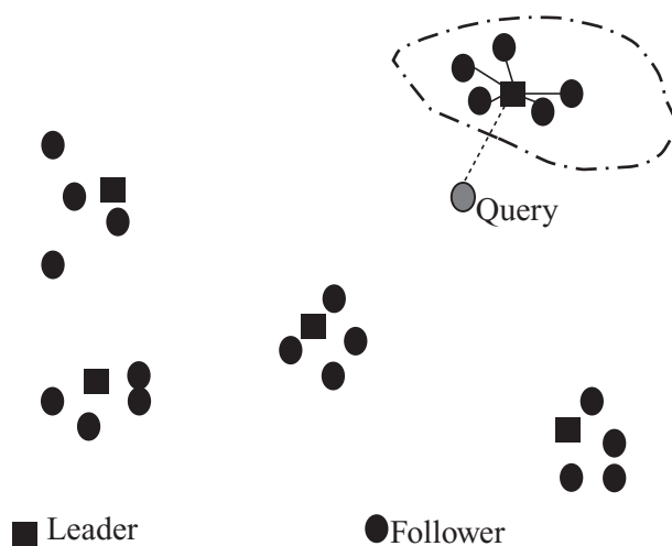
Figure 7.3 Cluster pruning.
